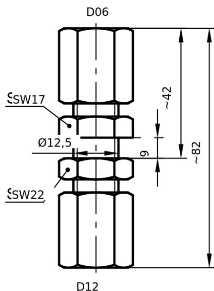
All data in mm; Illustration exemplary
