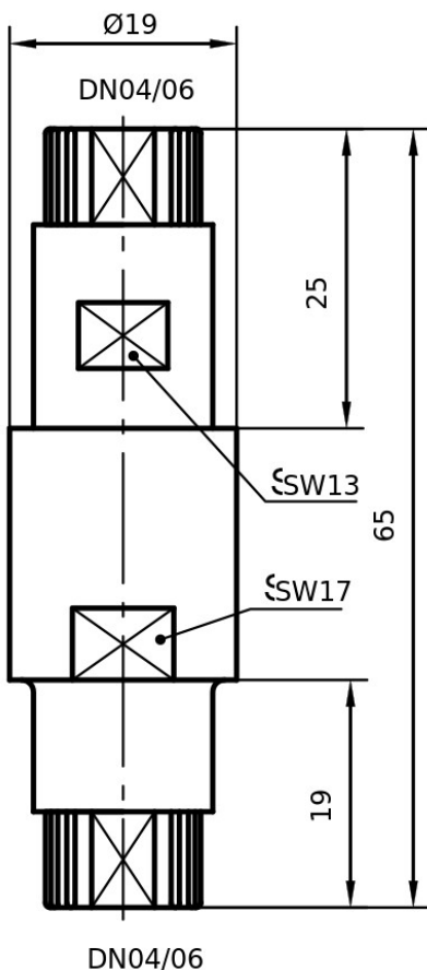
All data in mm; Illustration exemplary
