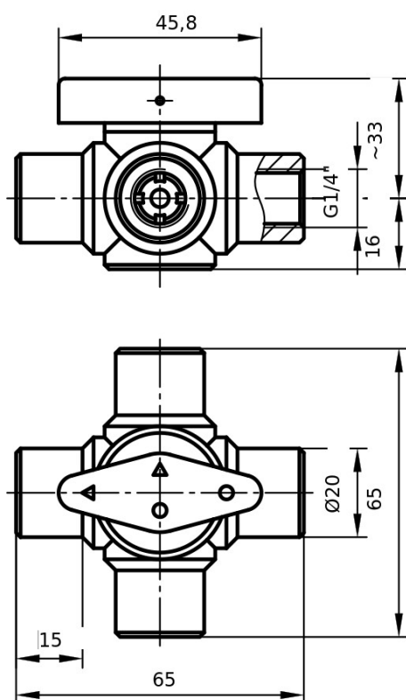
All data in mm; Illustration exemplary
