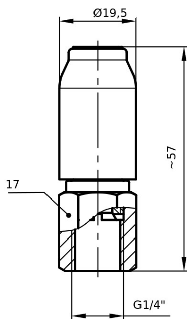
All data in mm; Illustration exemplary
