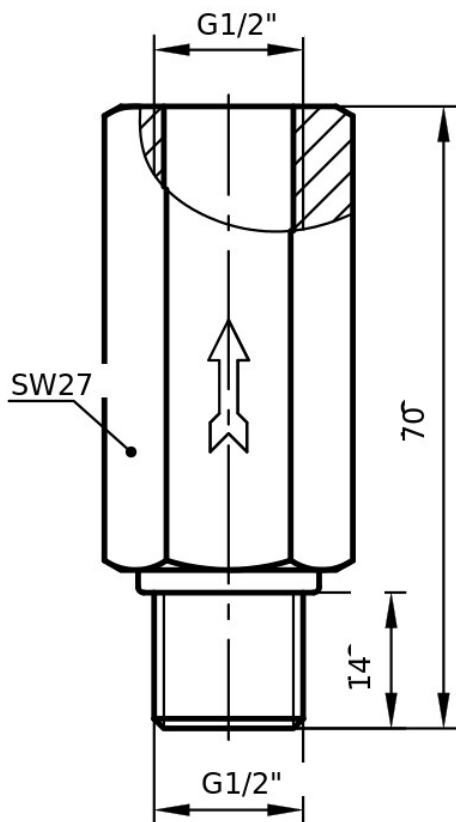
All data in mm; Illustration exemplary
